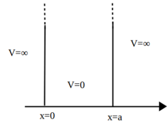
Fig: one dimensional infinite potential well.
