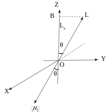
Fig: Orientation of angular momentum and magnetic diople moment of an electron in presence of an external magnetic field.
