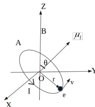
Fig: A magnetic moment in a magnetic field B.
